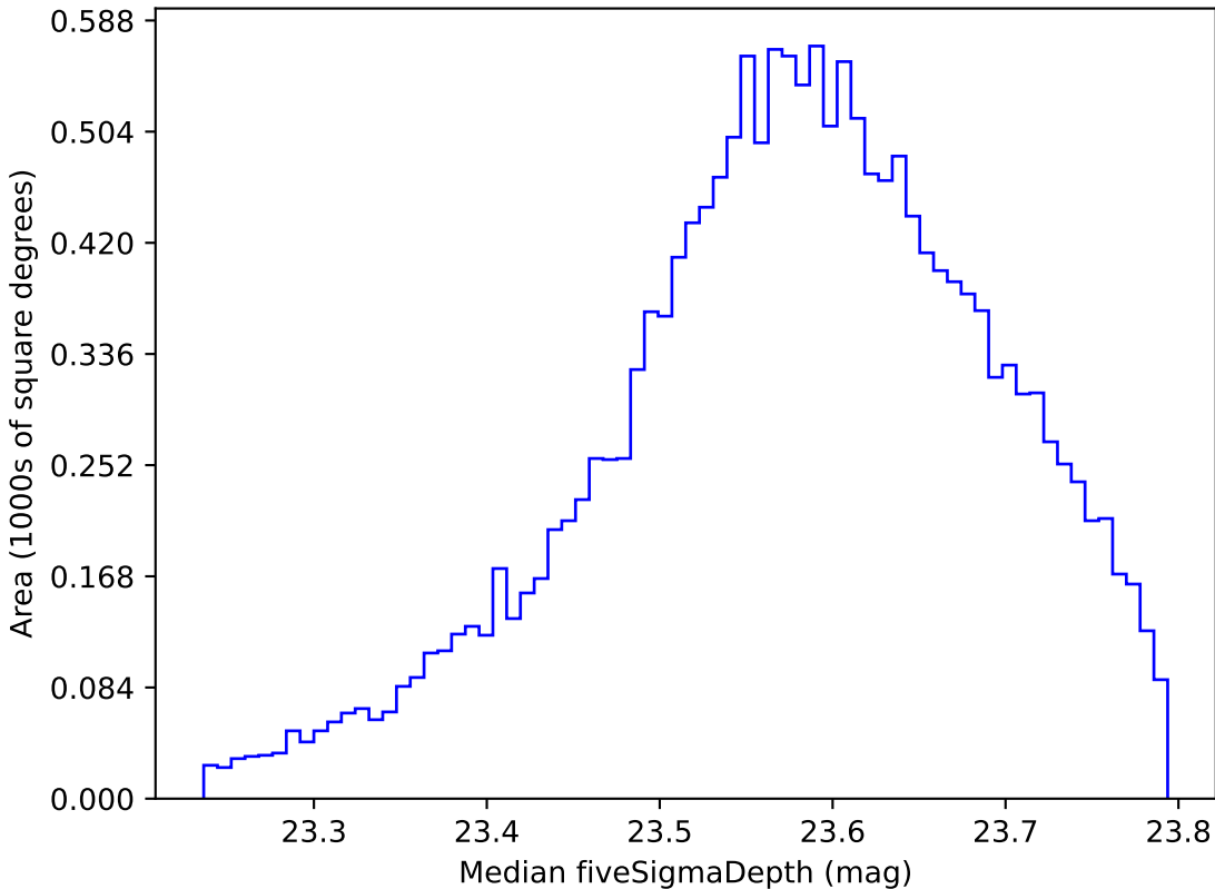
too_5_4v3.4_10yrs WFD i band: Median fiveSigmaDepth
