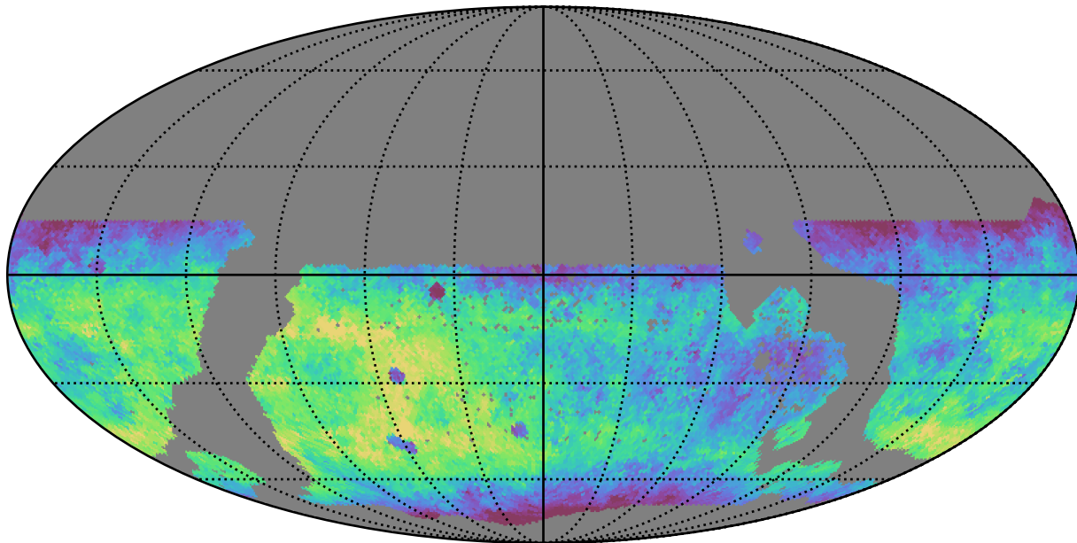
too_5_4v3.4_10yrs WFD g band: Median fiveSigmaDepth
