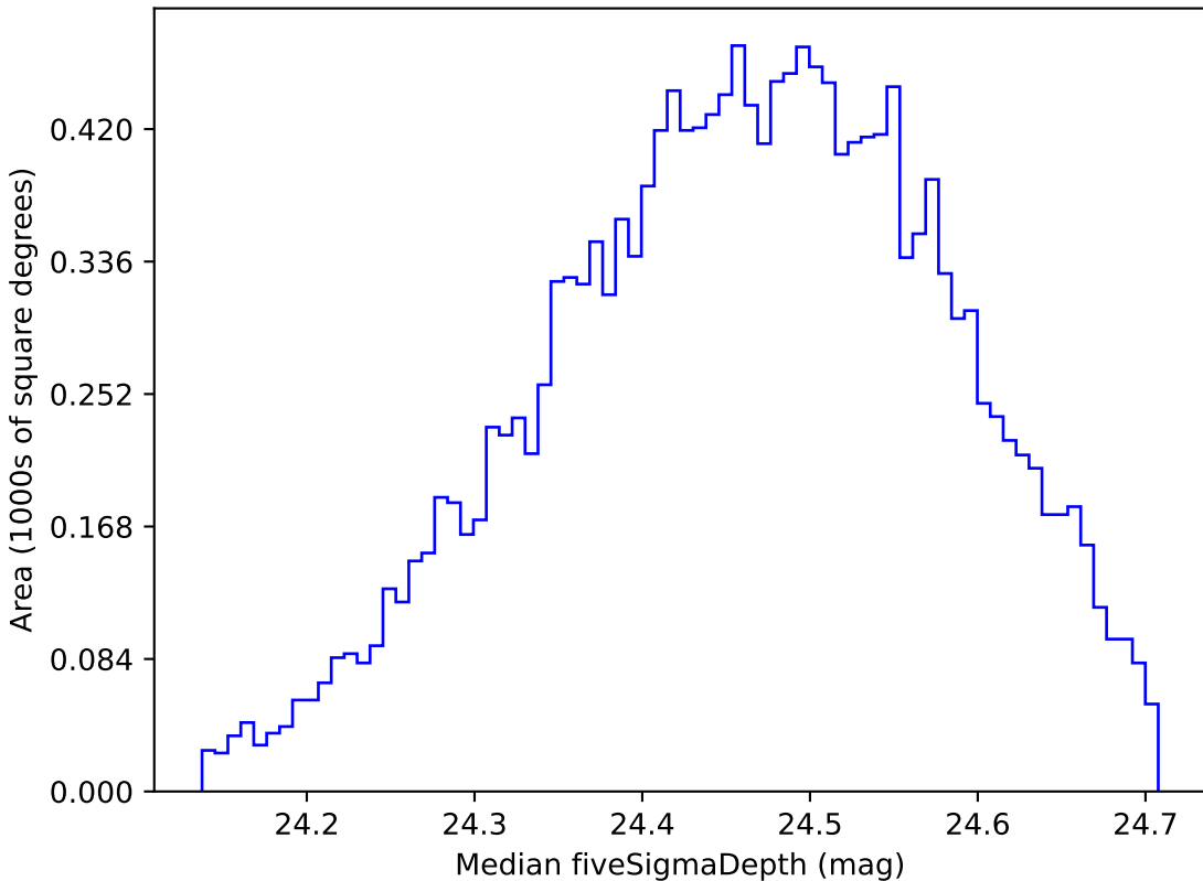
too_5_4v3.4_10yrs WFD g band: Median fiveSigmaDepth
