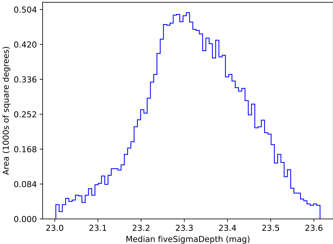
too_5_4v3.4_10yrs WFD all bands: Median fiveSigmaDepth
