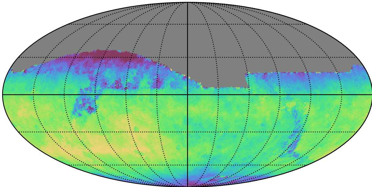
too_5_4v3.4_10yrs All sky z band: Median fiveSigmaDepth
