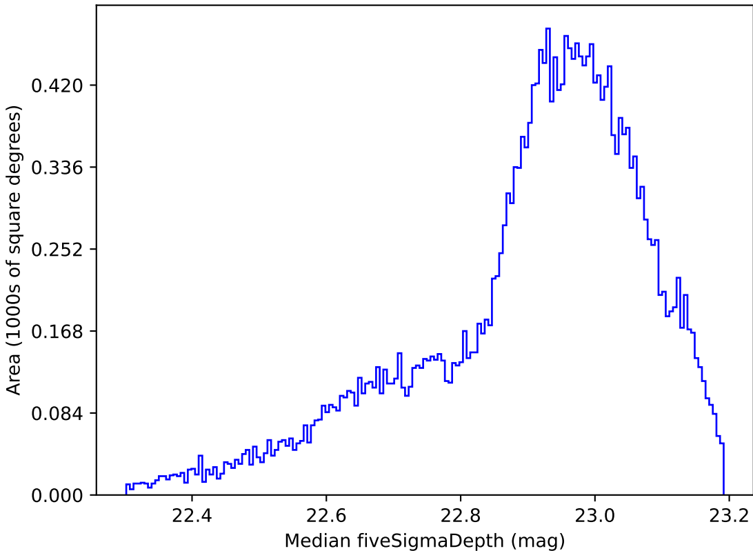
too_5_4v3.4_10yrs All sky z band: Median fiveSigmaDepth
