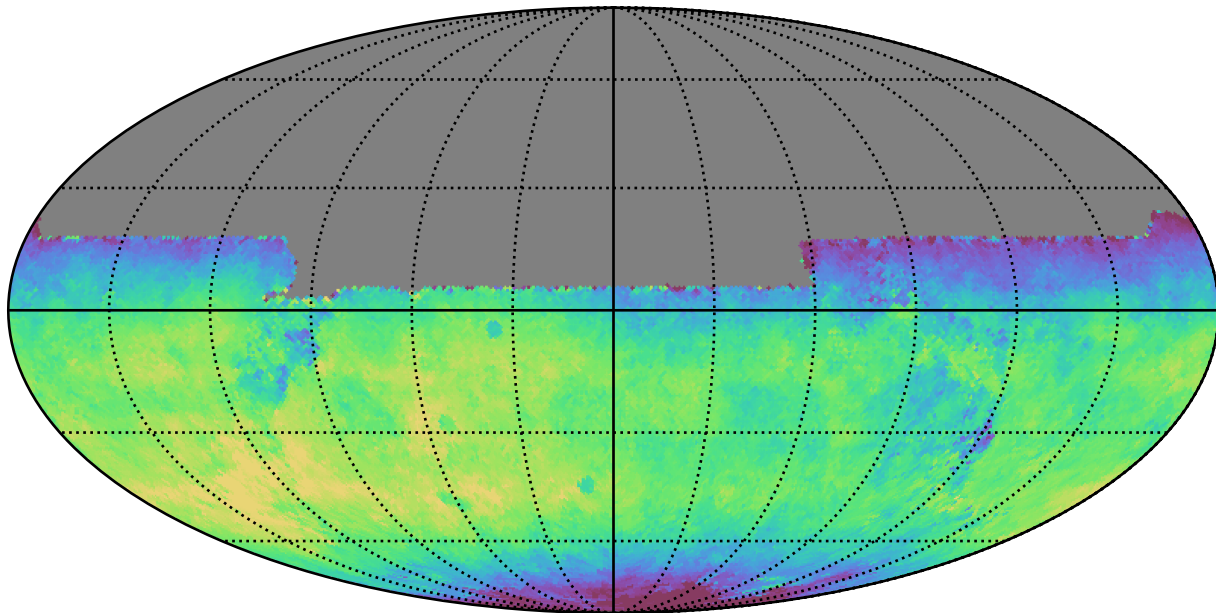
too_5_4v3.4_10yrs All sky y band: Median fiveSigmaDepth
