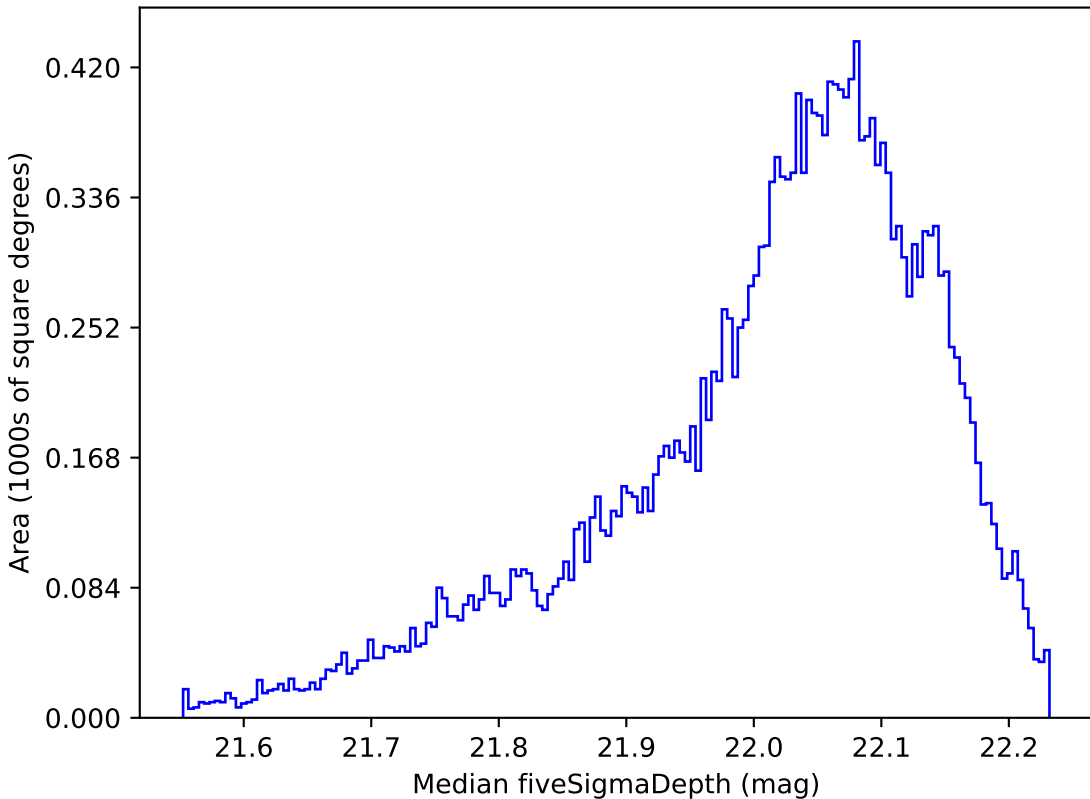
too_5_4v3.4_10yrs All sky y band: Median fiveSigmaDepth
