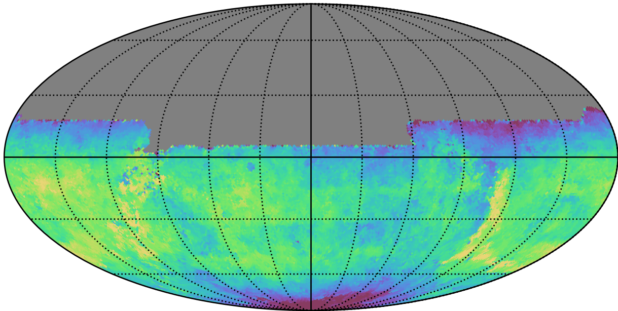
too_5_4v3.4_10yrs All sky u band: Median fiveSigmaDepth
