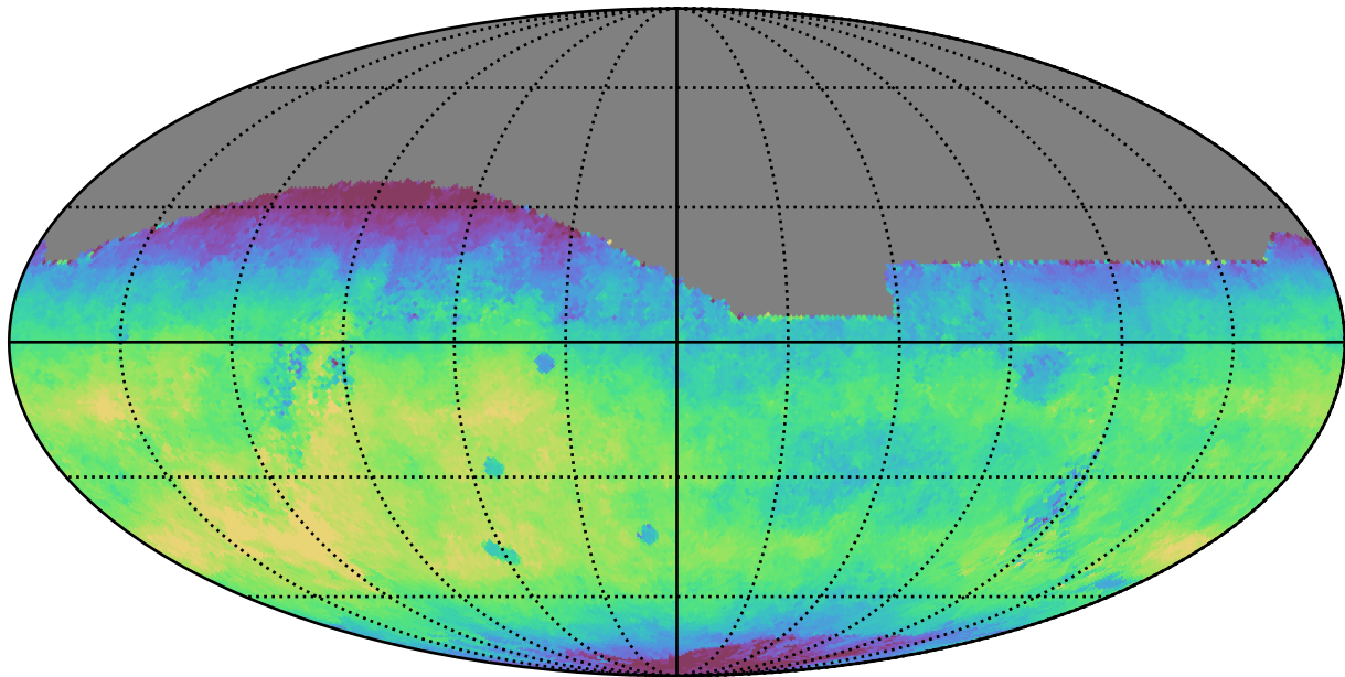
too_5_4v3.4_10yrs All sky r band: Median fiveSigmaDepth
