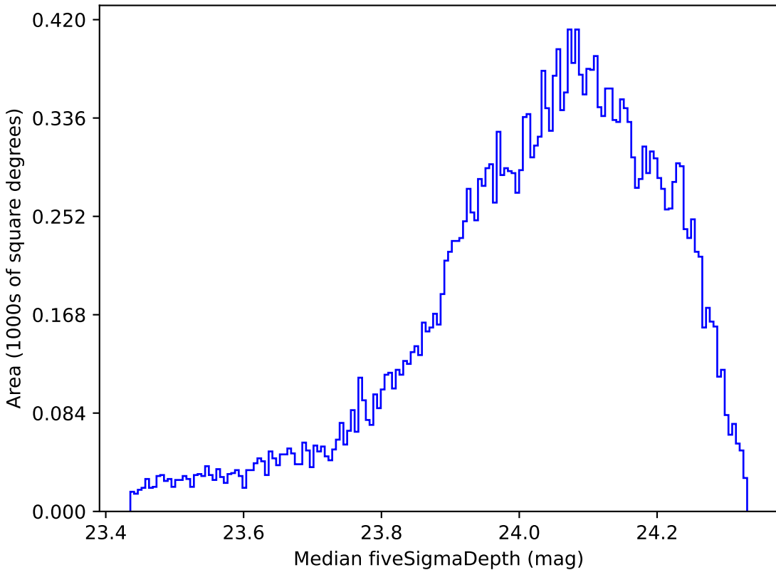
too_5_4v3.4_10yrs All sky r band: Median fiveSigmaDepth
