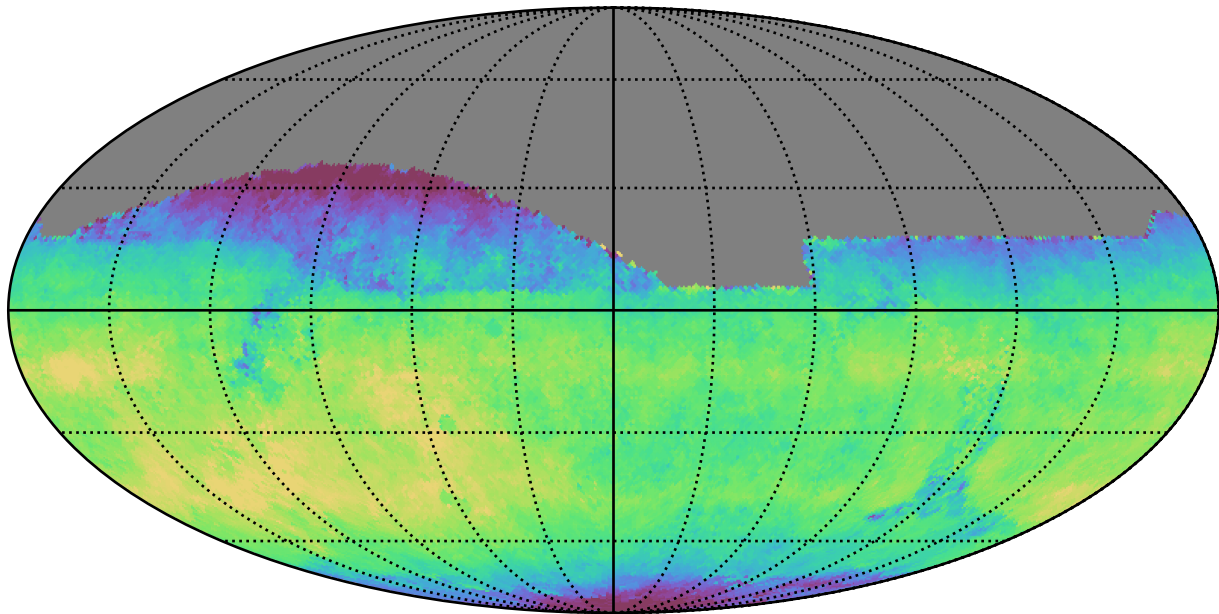
too_5_4v3.4_10yrs All sky i band: Median fiveSigmaDepth
