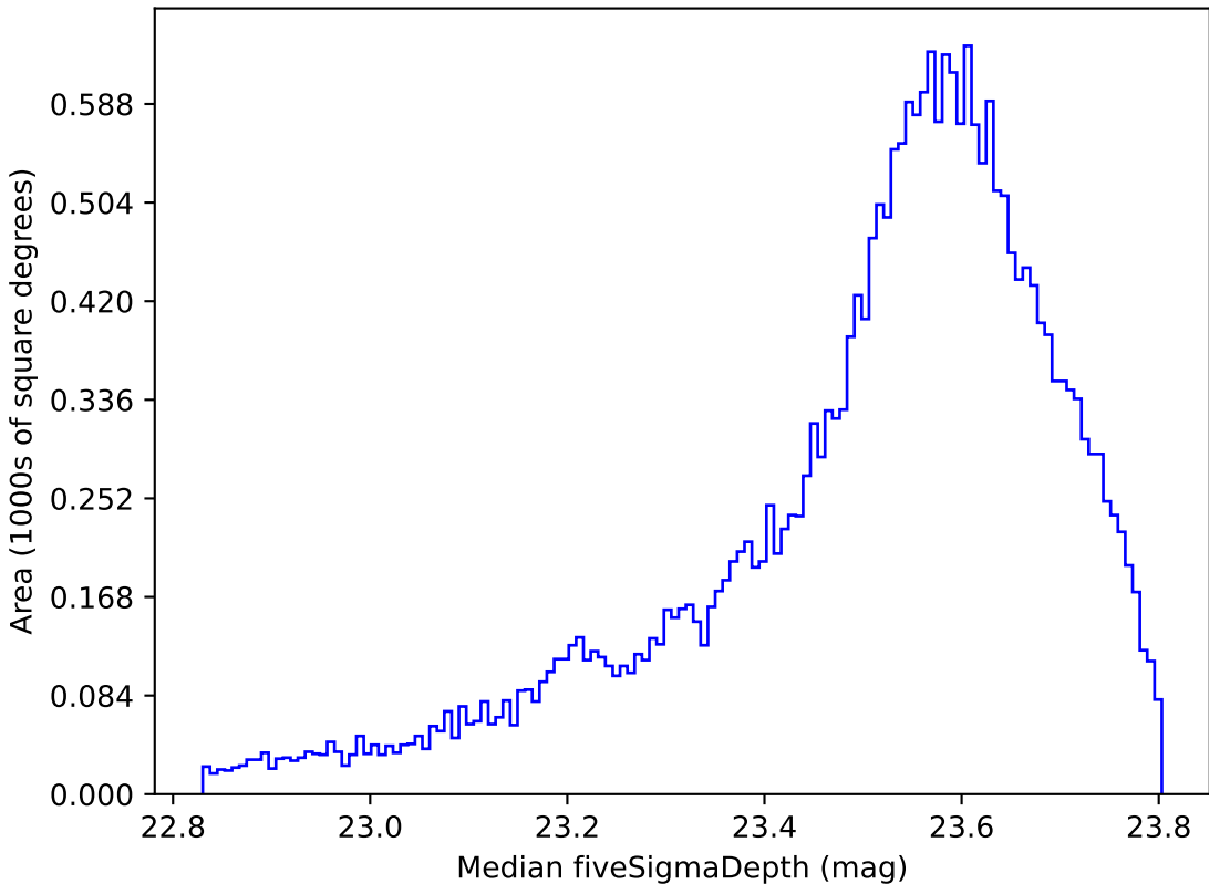
too_5_4v3.4_10yrs All sky i band: Median fiveSigmaDepth
