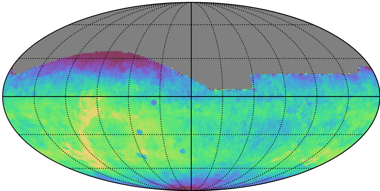
too_5_4v3.4_10yrs All sky g band: Median fiveSigmaDepth
