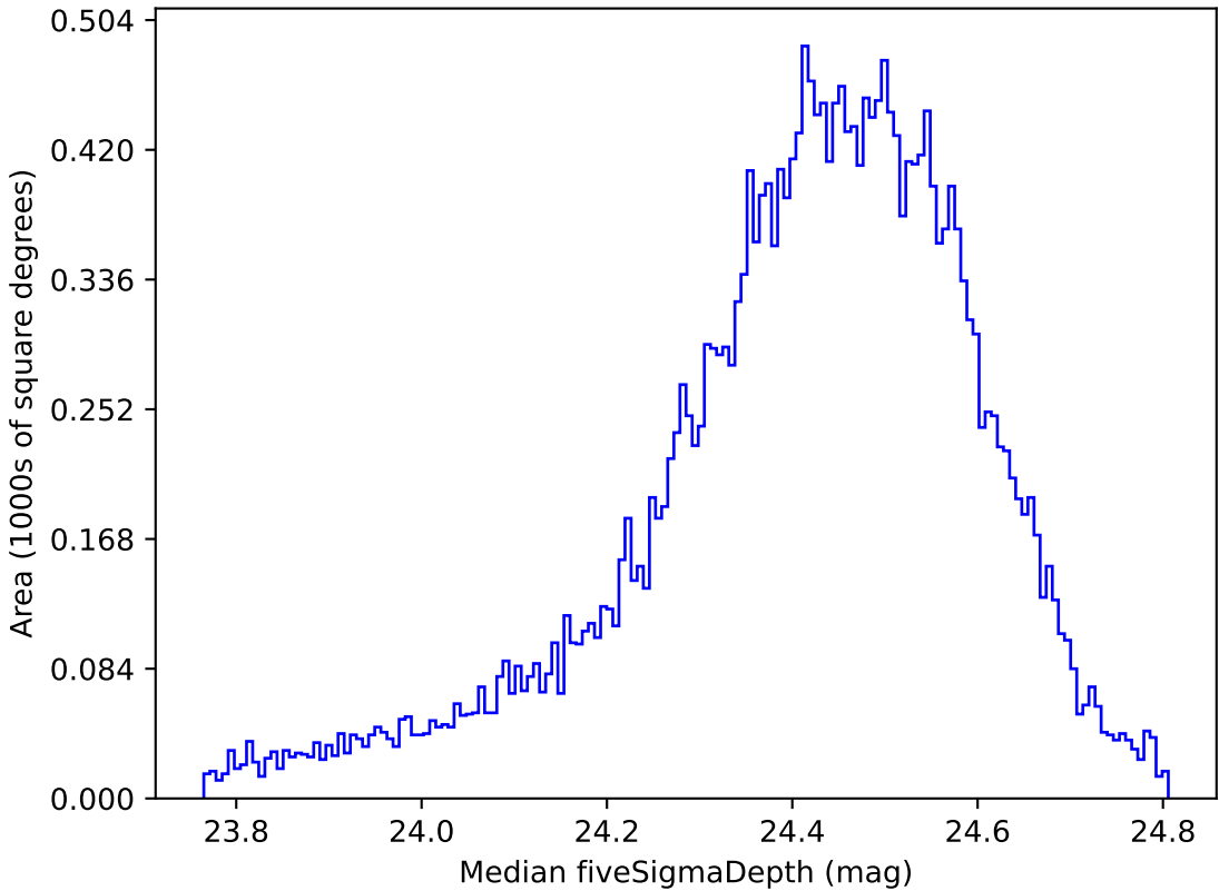
too_5_4v3.4_10yrs All sky g band: Median fiveSigmaDepth
