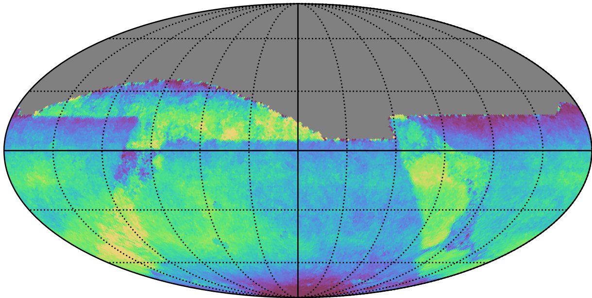
too_5_4v3.4_10yrs All sky all bands: Median fiveSigmaDepth
