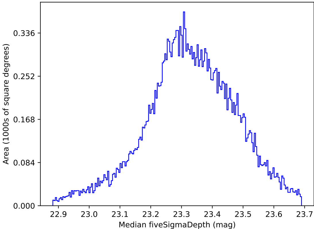
too_5_4v3.4_10yrs All sky all bands: Median fiveSigmaDepth
