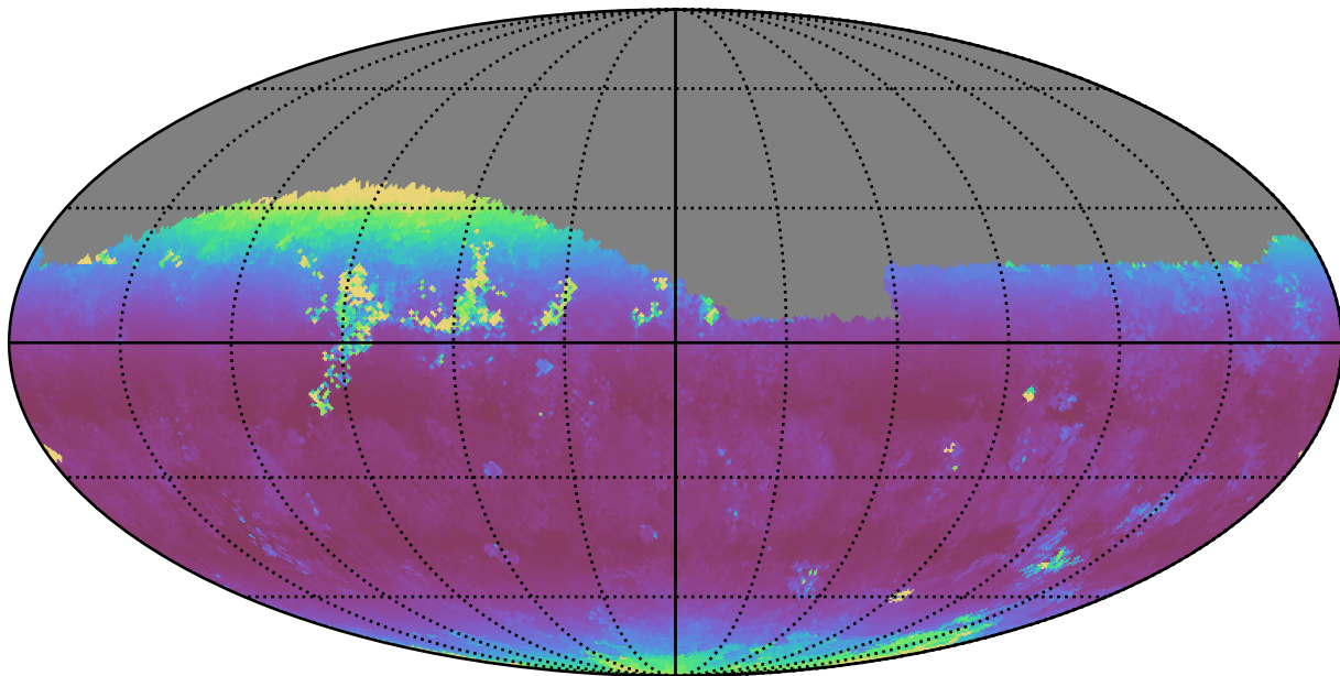
too_5_4v3.4_10yrs Yr 1 z band: Median airmass
