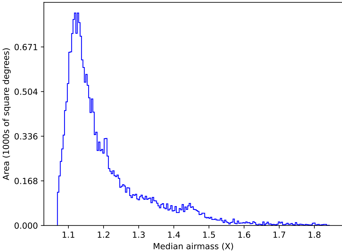
too_5_4v3.4_10yrs Yr 1 y band: Median airmass
