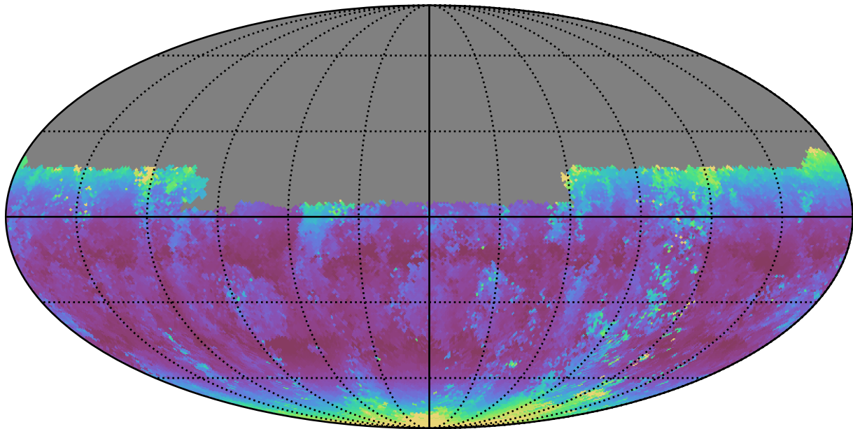
too_5_4v3.4_10yrs Yr 1 u band: Median airmass
