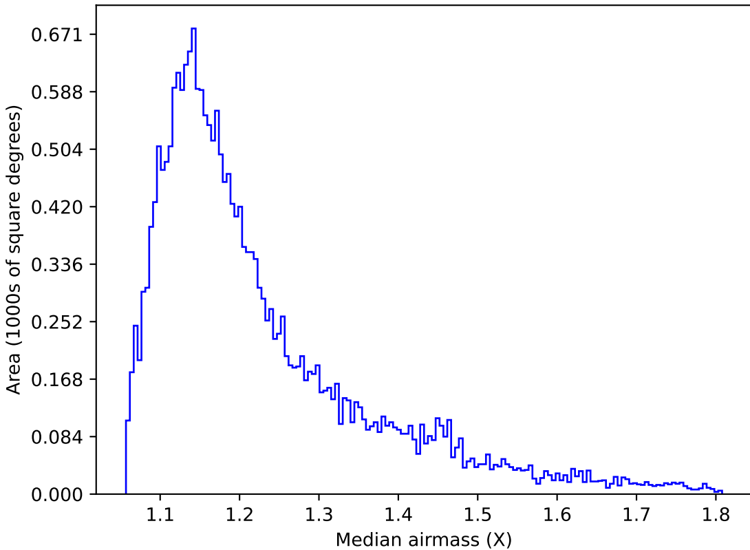
too_5_4v3.4_10yrs Yr 1 u band: Median airmass
