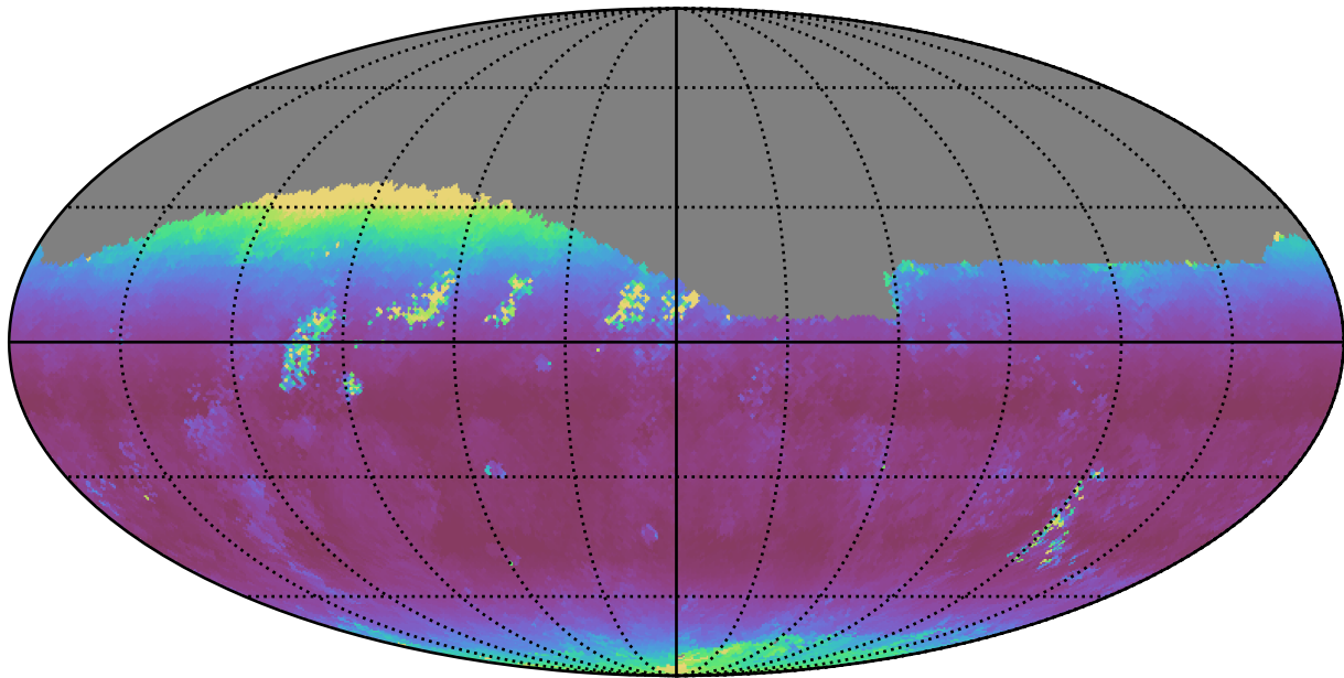
too_5_4v3.4_10yrs Yr 1 r band: Median airmass
