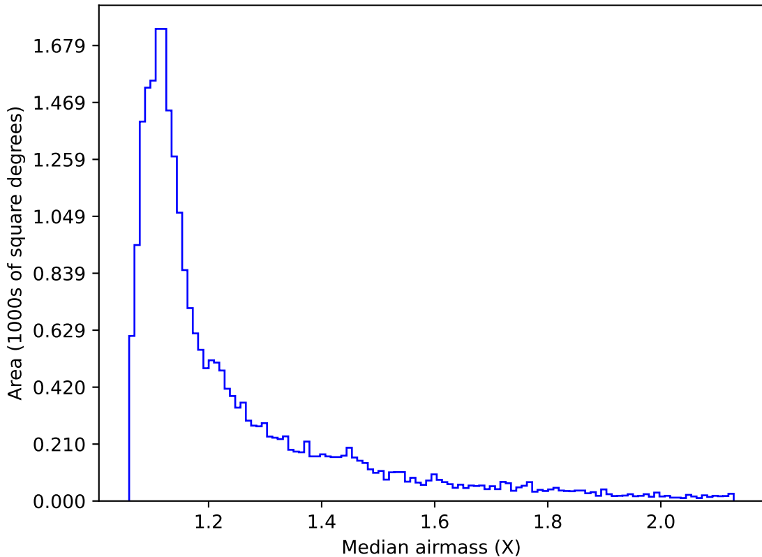
too_5_4v3.4_10yrs Yr 1 r band: Median airmass
