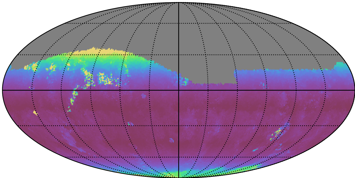
too_5_4v3.4_10yrs Yr 1 i band: Median airmass
