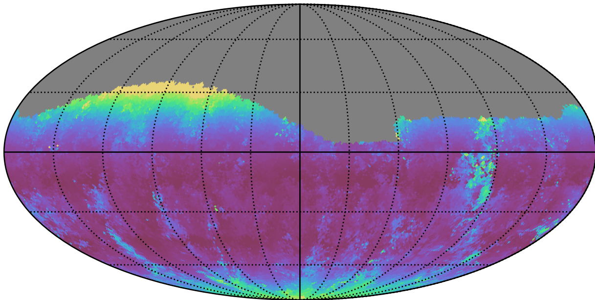
too_5_4v3.4_10yrs Yr 1 g band: Median airmass
