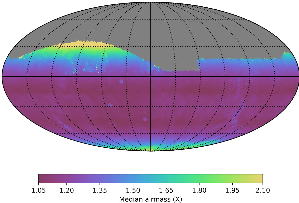
too_5_4v3.4_10yrs Yr 1 all bands: Median airmass
