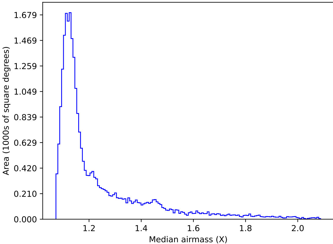
too_5_4v3.4_10yrs Yr 1 all bands: Median airmass
