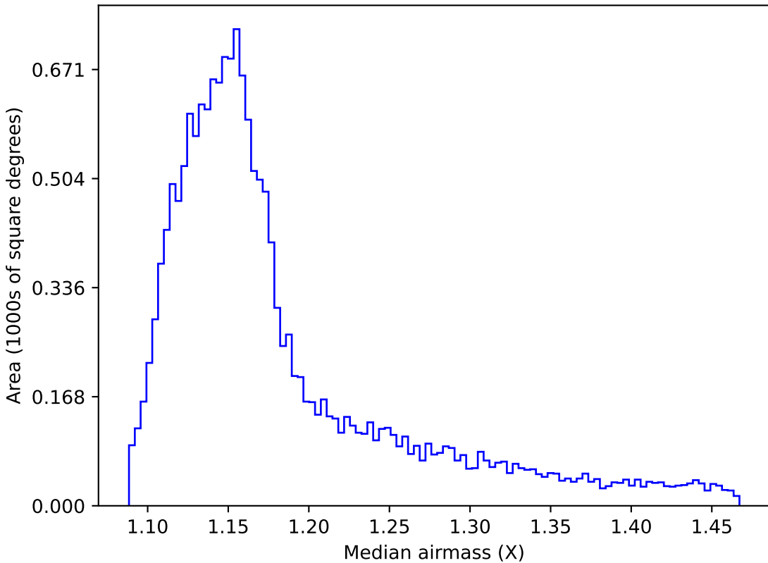
too_5_4v3.4_10yrs WFD z band: Median airmass
