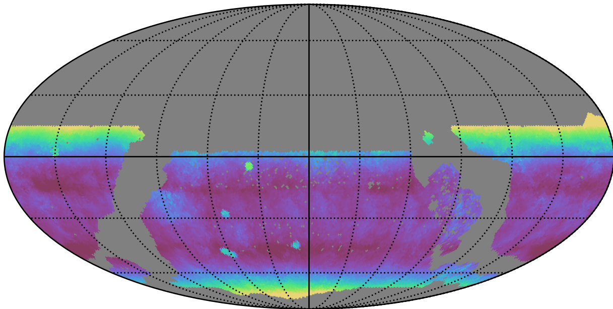
too_5_4v3.4_10yrs WFD y band: Median airmass
