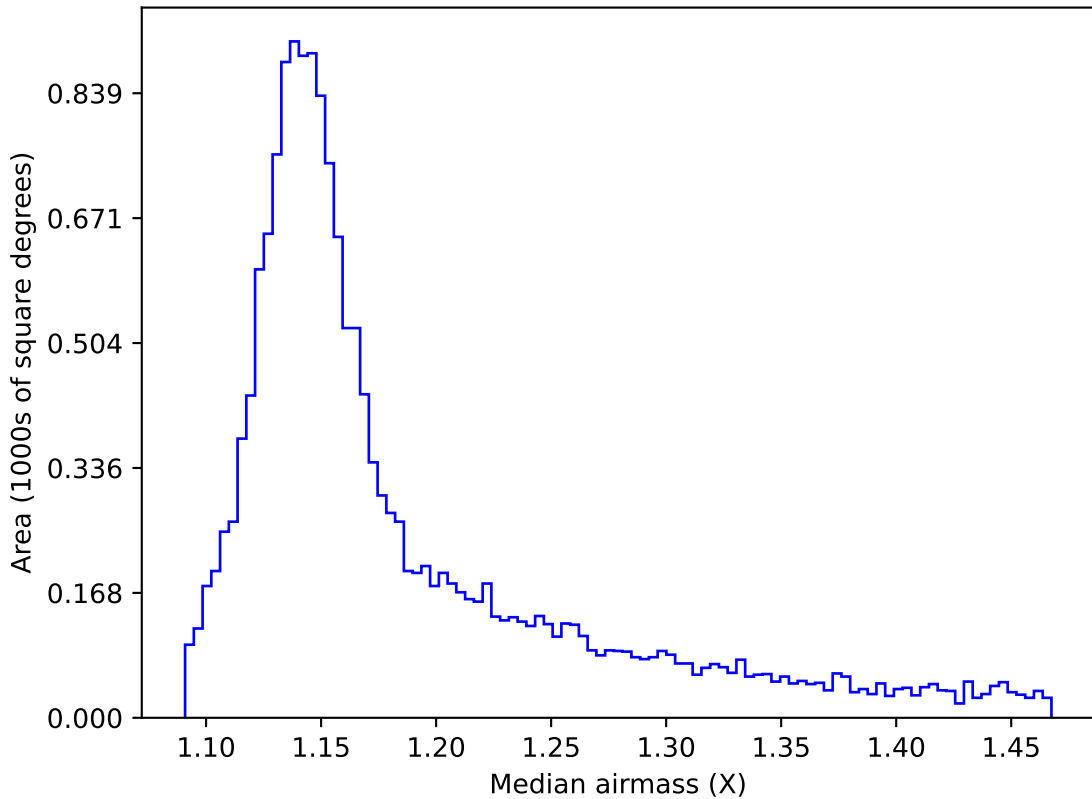
too_5_4v3.4_10yrs WFD y band: Median airmass
