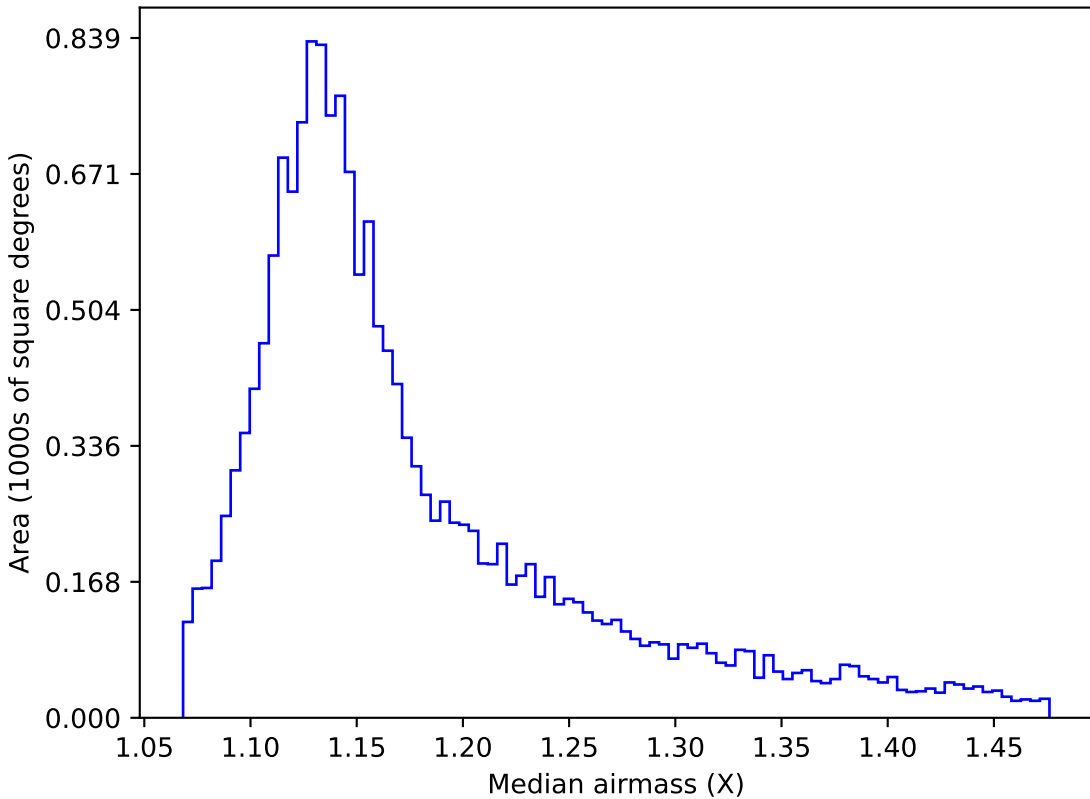
too_5_4v3.4_10yrs WFD u band: Median airmass
