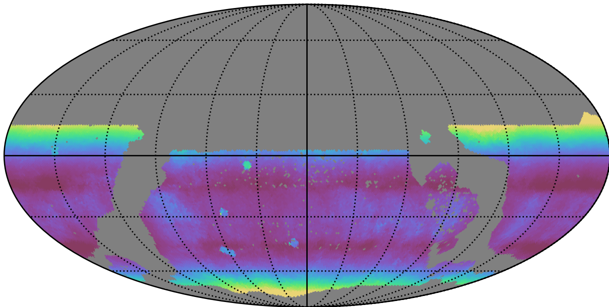
too_5_4v3.4_10yrs WFD r band: Median airmass
