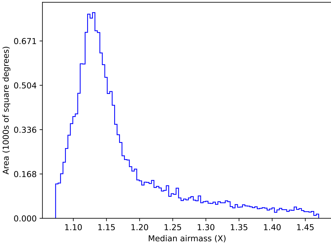
too_5_4v3.4_10yrs WFD r band: Median airmass
