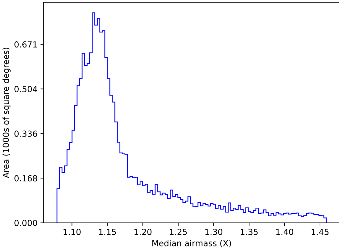
too_5_4v3.4_10yrs WFD i band: Median airmass
