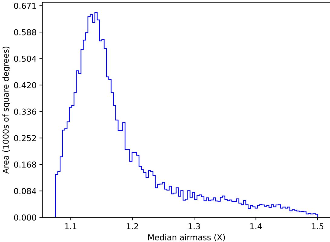
too_5_4v3.4_10yrs WFD g band: Median airmass
