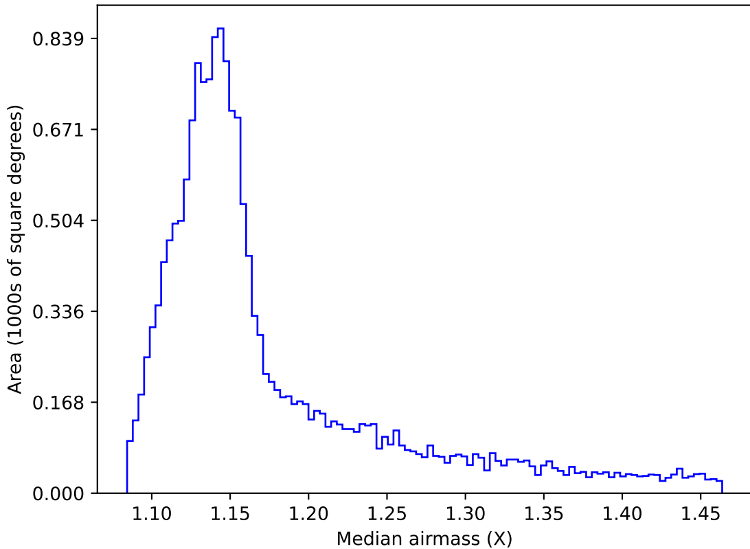
too_5_4v3.4_10yrs WFD all bands: Median airmass
