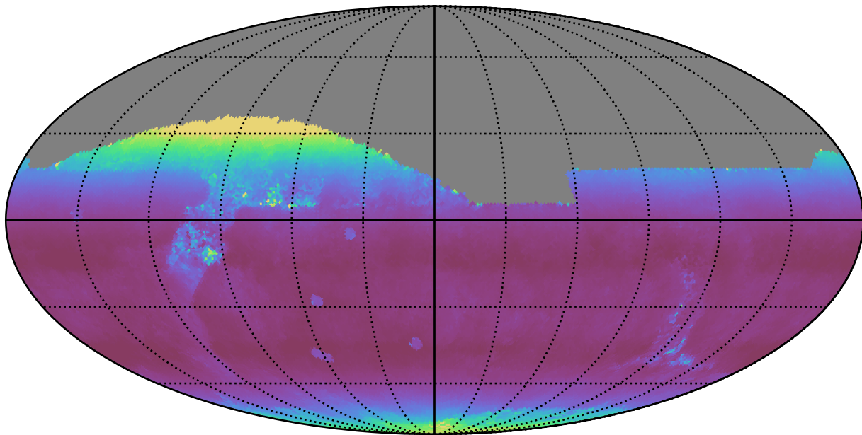
too_5_4v3.4_10yrs All sky z band: Median airmass
