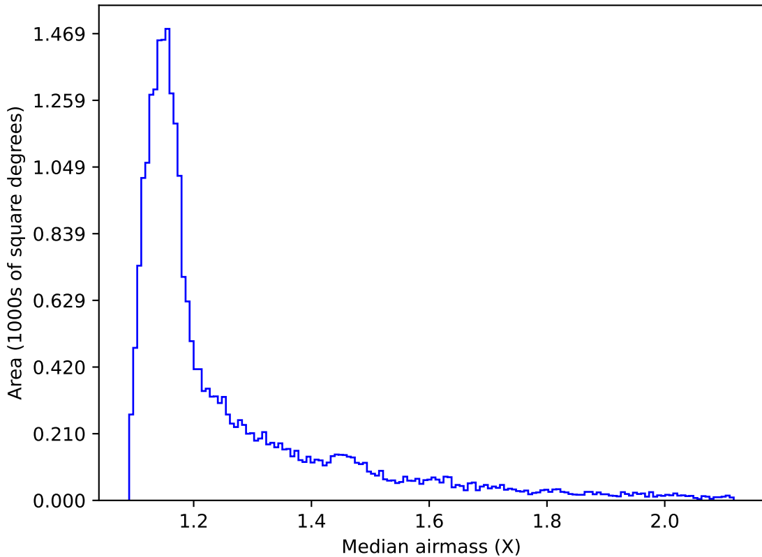
too_5_4v3.4_10yrs All sky z band: Median airmass
