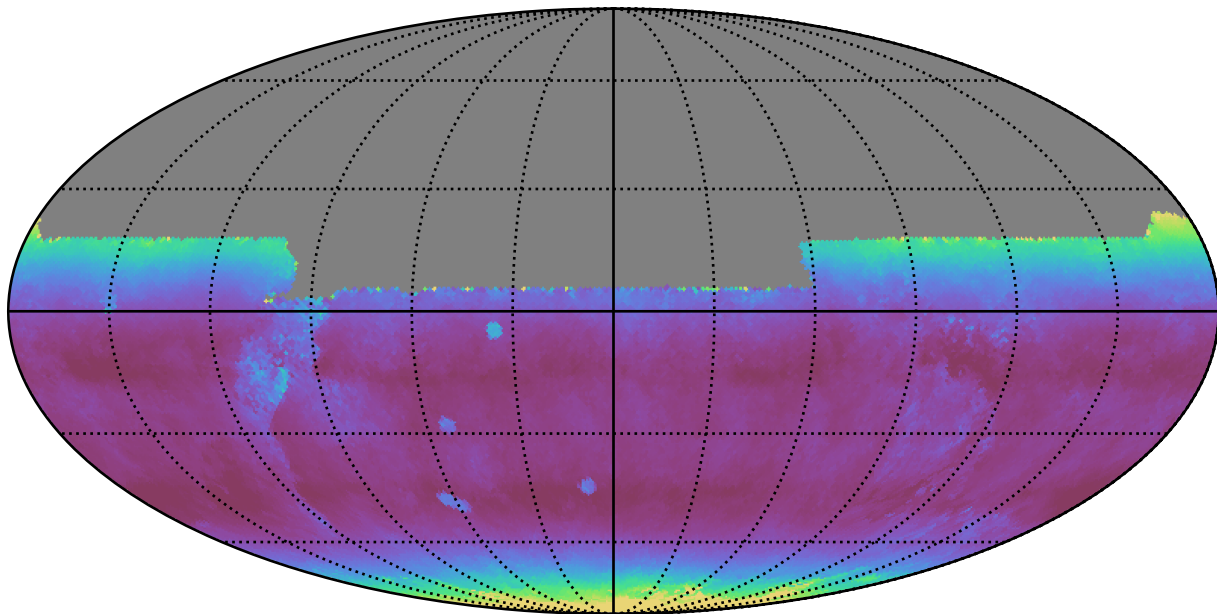
too_5_4v3.4_10yrs All sky y band: Median airmass
