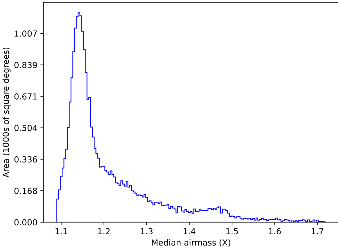
too_5_4v3.4_10yrs All sky y band: Median airmass
