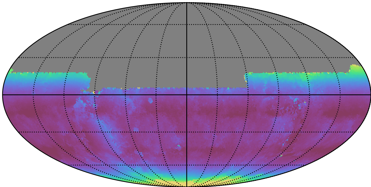
too_5_4v3.4_10yrs All sky u band: Median airmass
