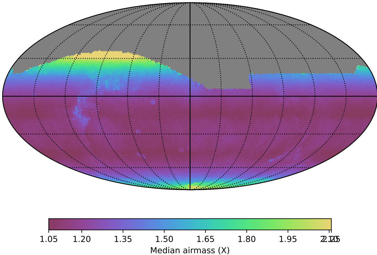
too_5_4v3.4_10yrs All sky i band: Median airmass
