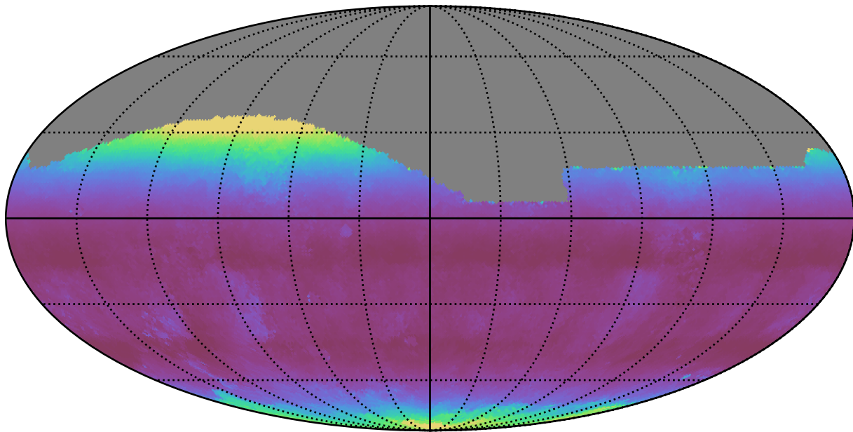
too_5_4v3.4_10yrs All sky g band: Median airmass
