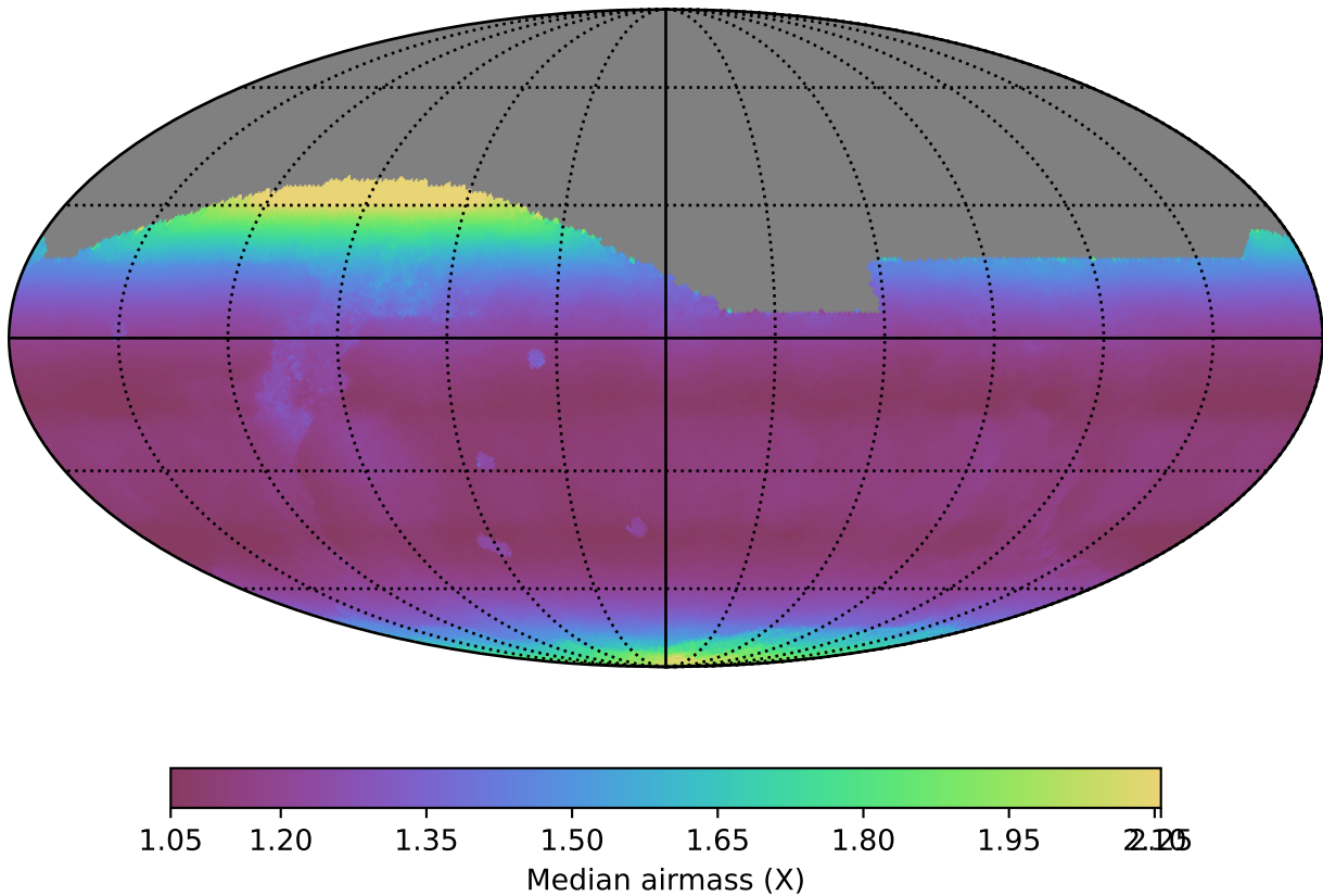
too_5_4v3.4_10yrs All sky all bands: Median airmass
