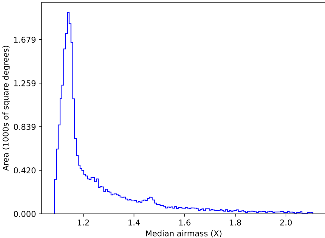
too_5_4v3.4_10yrs All sky all bands: Median airmass
