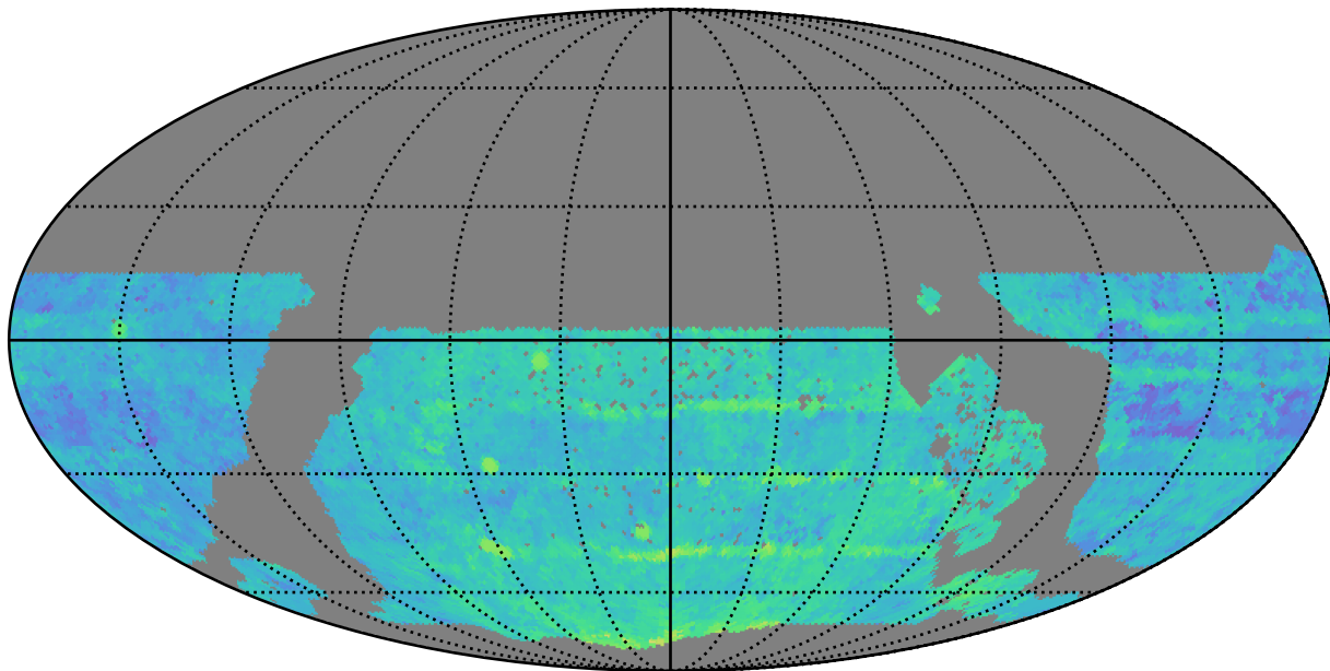
too_5_4v3.4_10yrs WFD z band: Median Season Length
