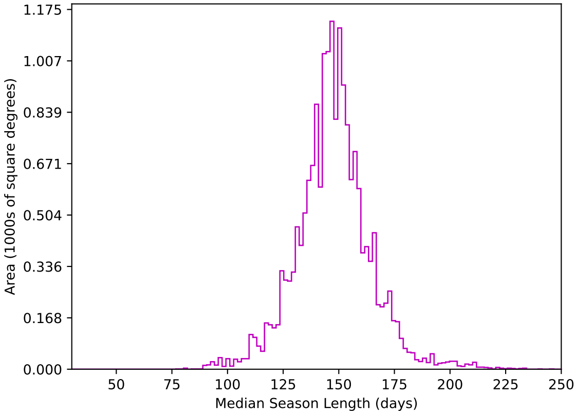
too_5_4v3.4_10yrs WFD z band: Median Season Length
