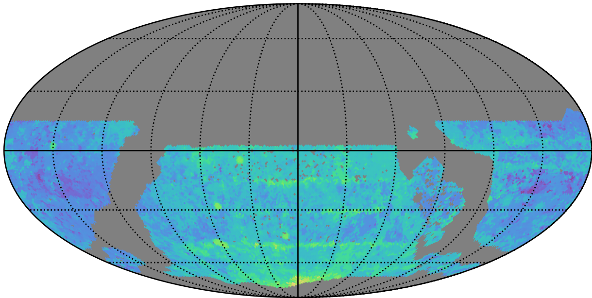
too_5_4v3.4_10yrs WFD y band: Median Season Length
