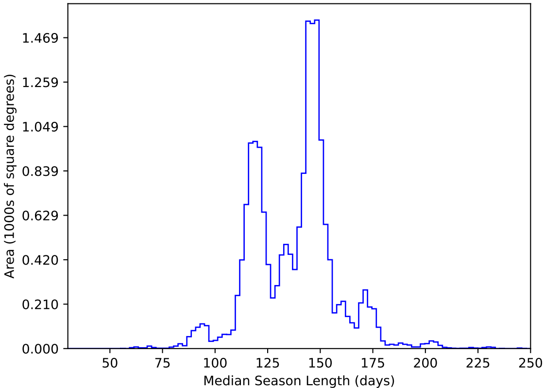
too_5_4v3.4_10yrs WFD y band: Median Season Length
