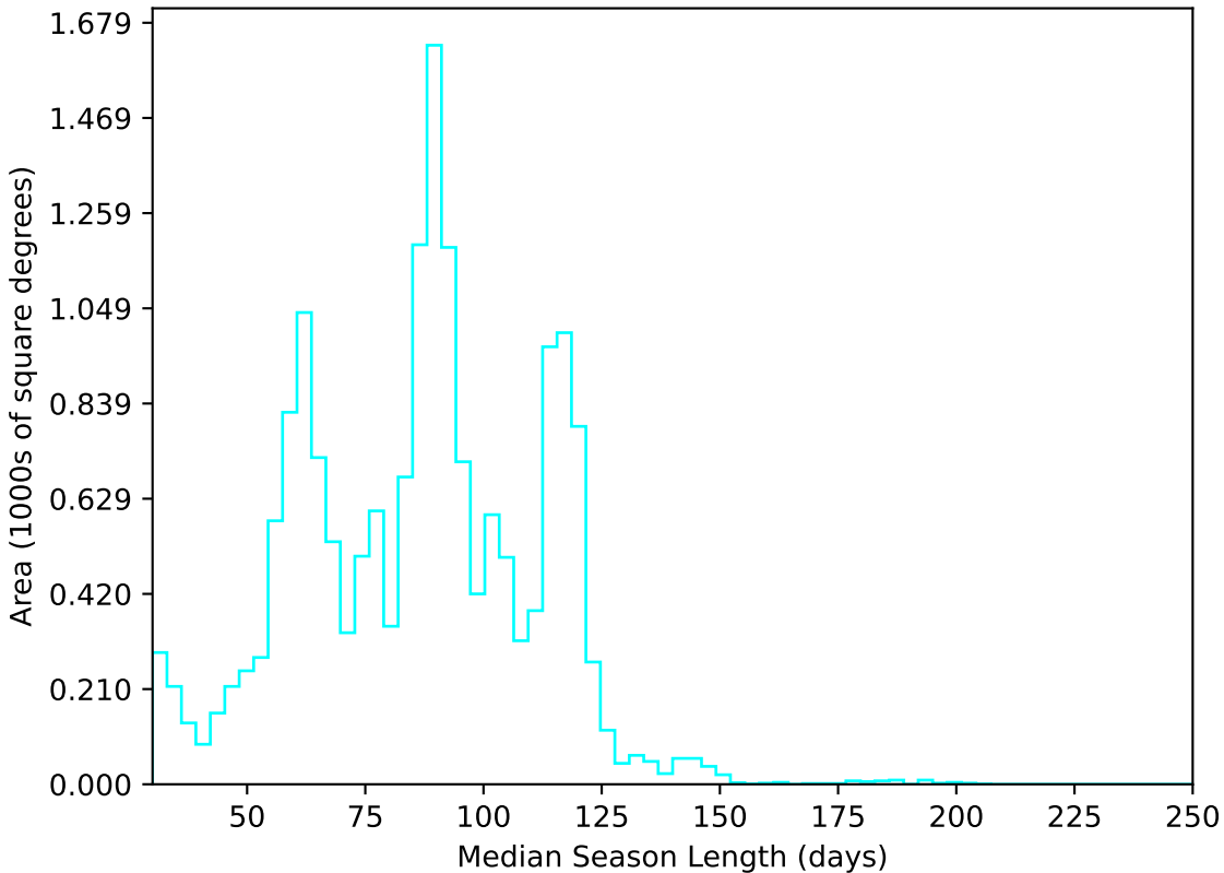
too_5_4v3.4_10yrs WFD u band: Median Season Length
